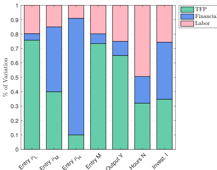
FIGURE 12: VARIANCE DECOMPOSITION
